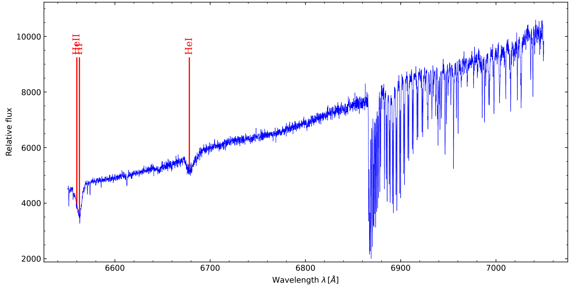
Xi Persei - O7.5 III (6550 - 7050 Å, orders merged by PYTHON)
