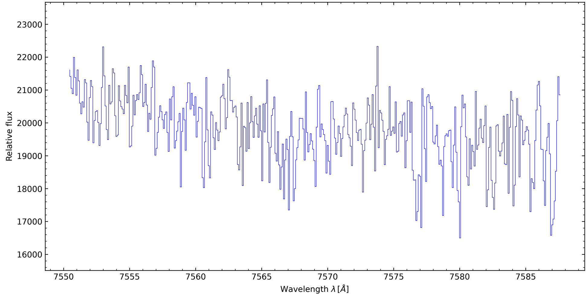
Xi Persei - O7.5 III (7550 - 7587 Å, orders merged by PYTHON)
