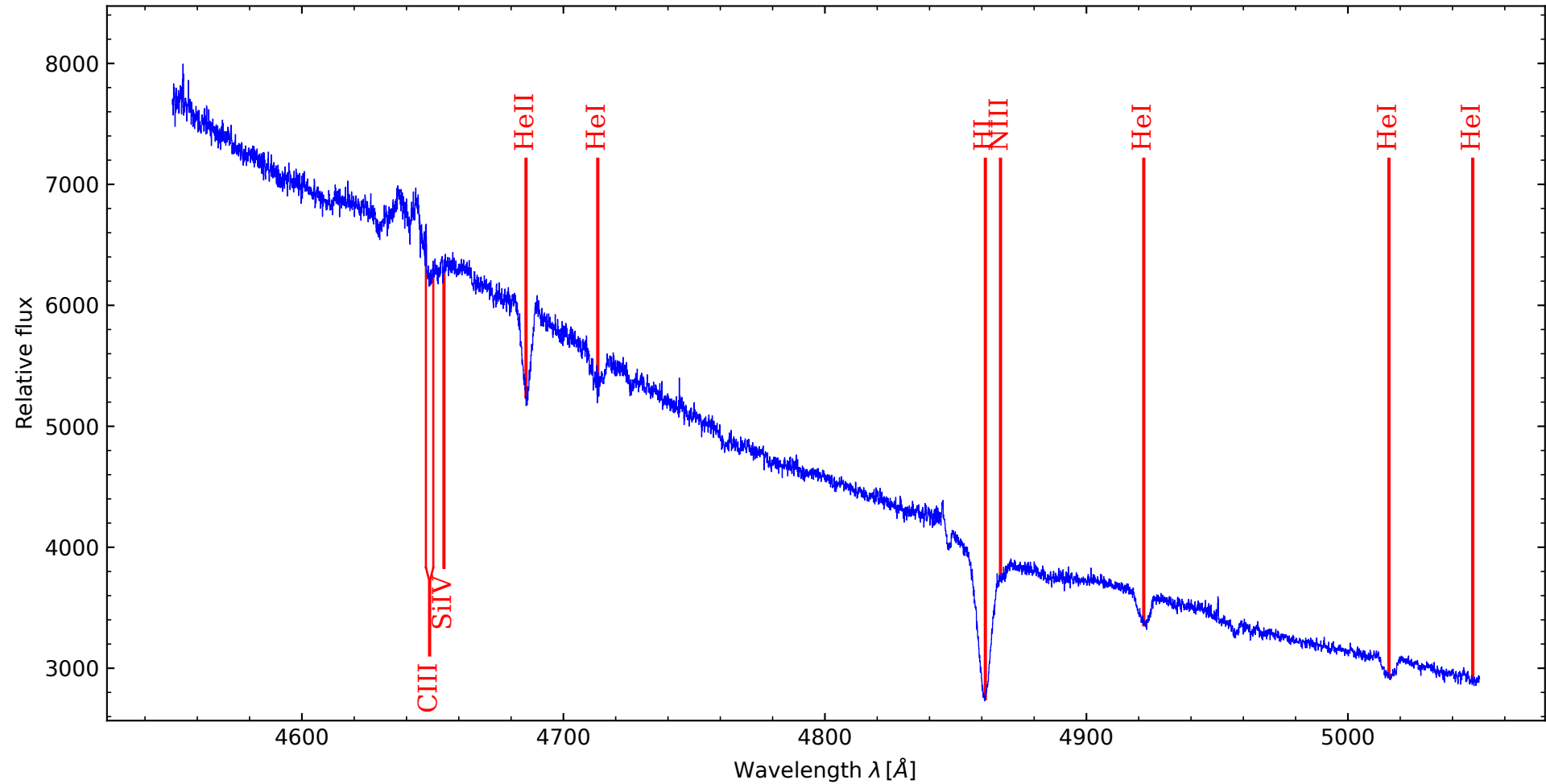
Xi Persei - O7.5 III (4550 - 5050 Å, orders merged by PYTHON)
