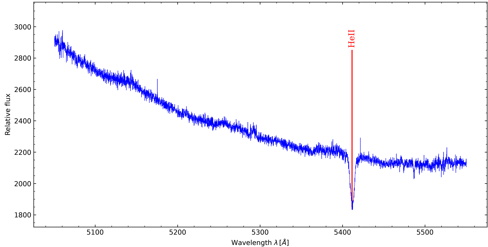
Xi Persei - O7.5 III (5050 - 5550 Å, orders merged by PYTHON)
