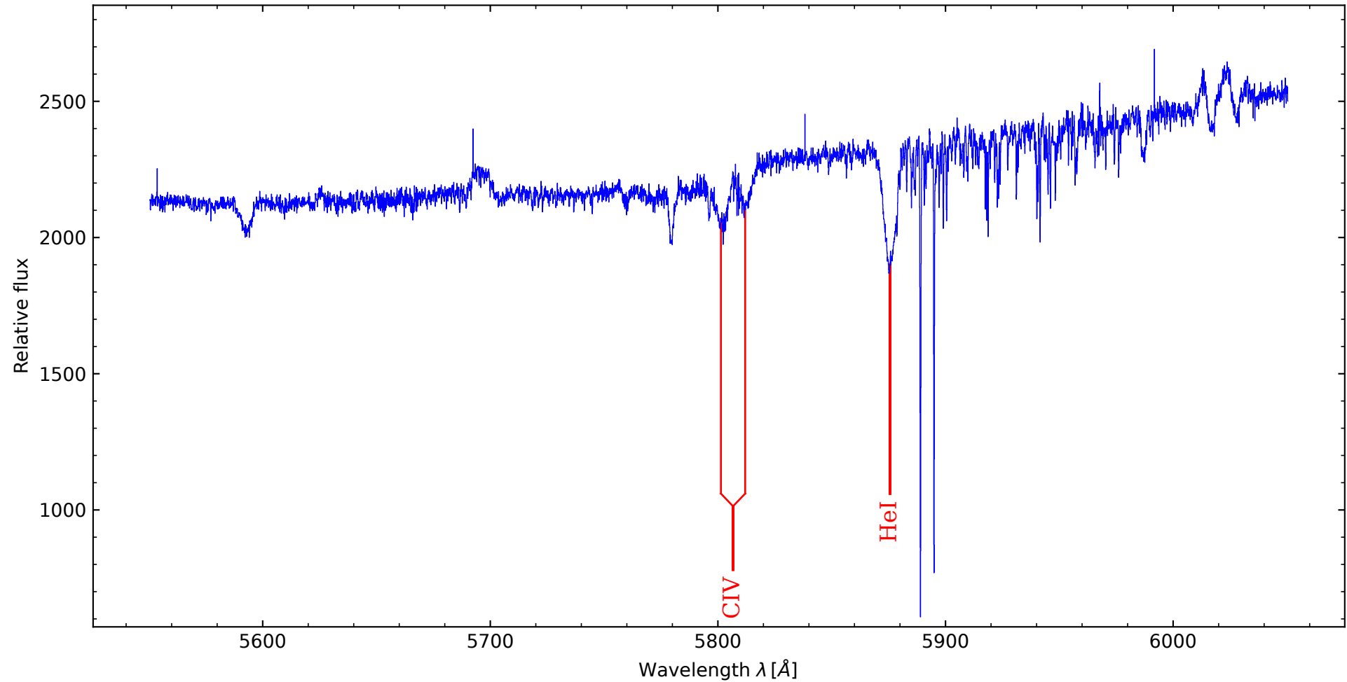
Xi Persei - O7.5 III (5550 - 6050 Å, orders merged by PYTHON)
