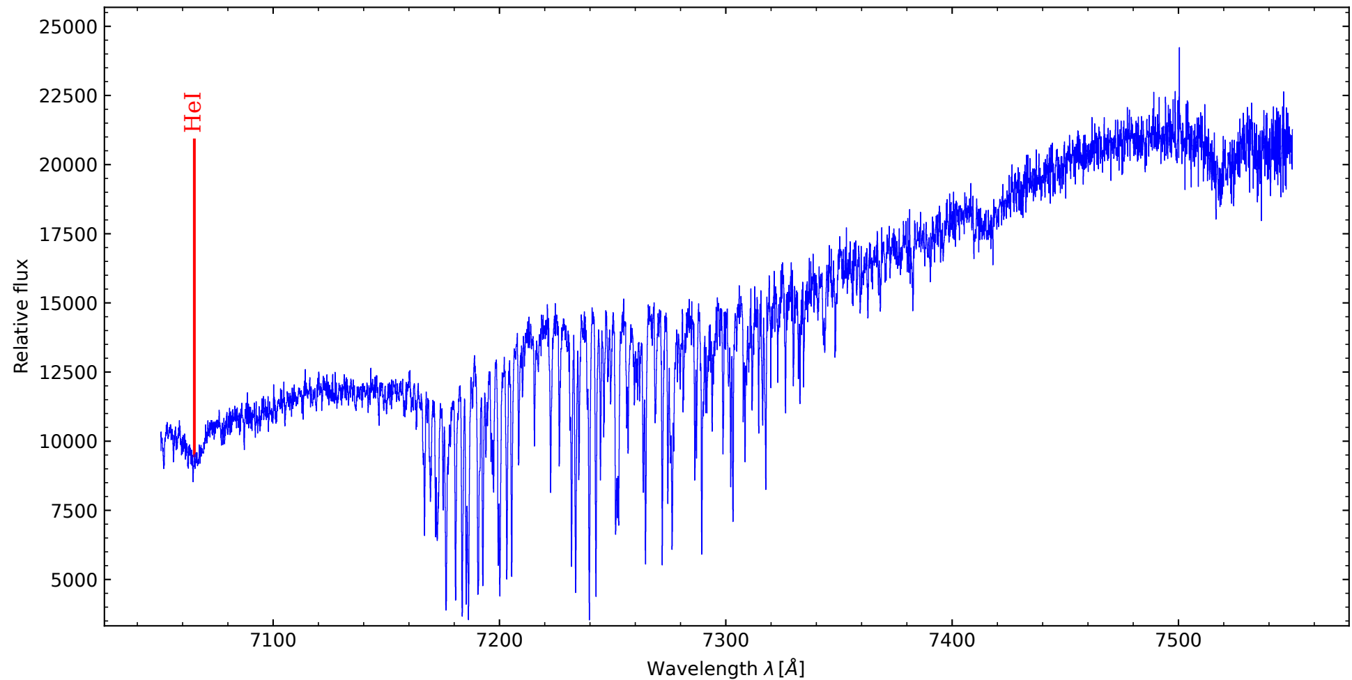
Xi Persei - O7.5 III (7050 - 7550 Å, orders merged by PYTHON)
