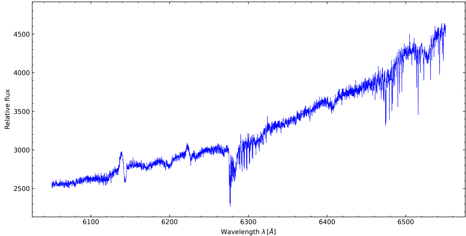
Xi Persei - O7.5 III (6050 - 6550 Å, orders merged by PYTHON)
