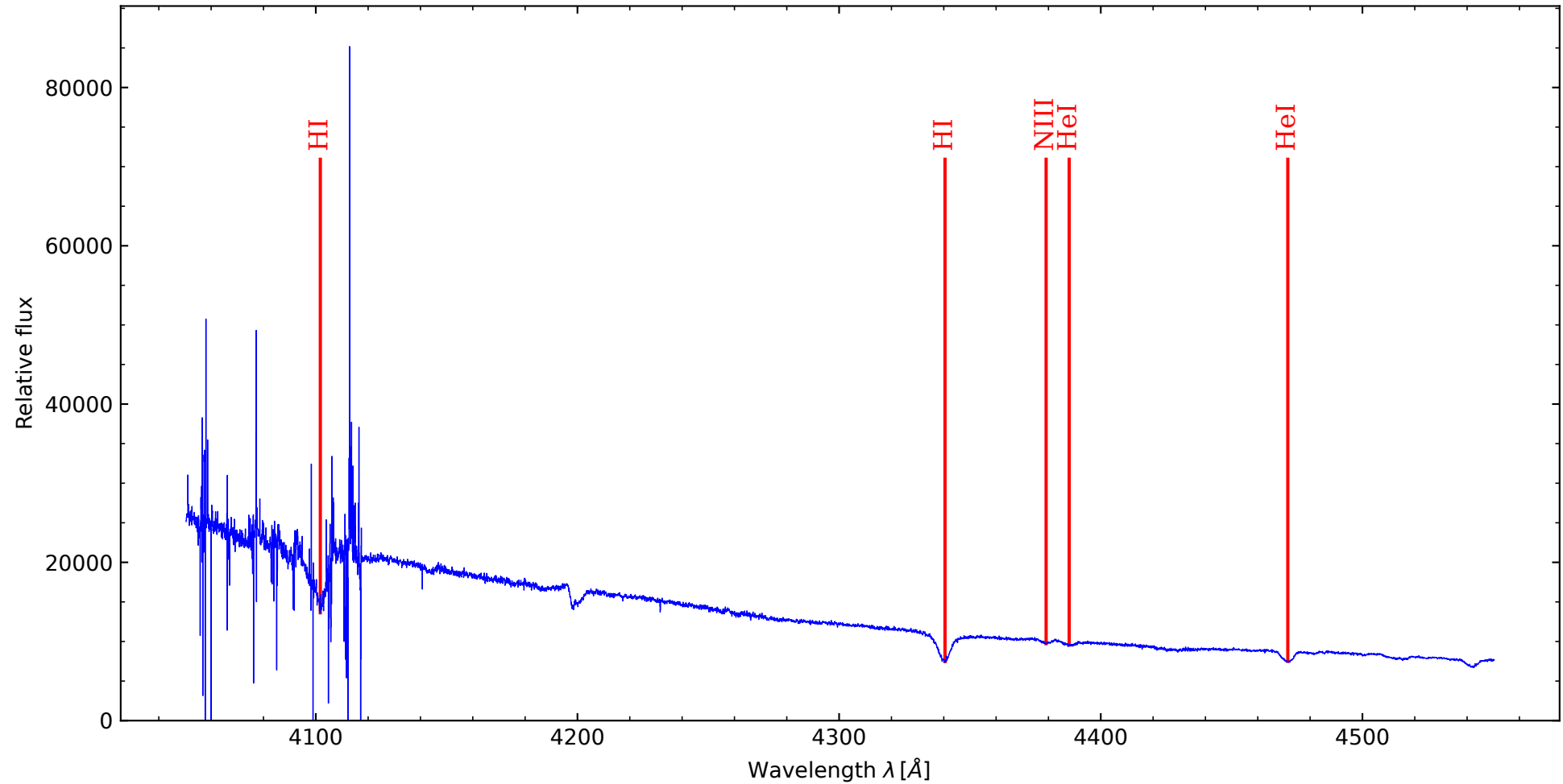
Xi Persei - O7.5 III (4050 - 4550 Å, orders merged by PYTHON)
