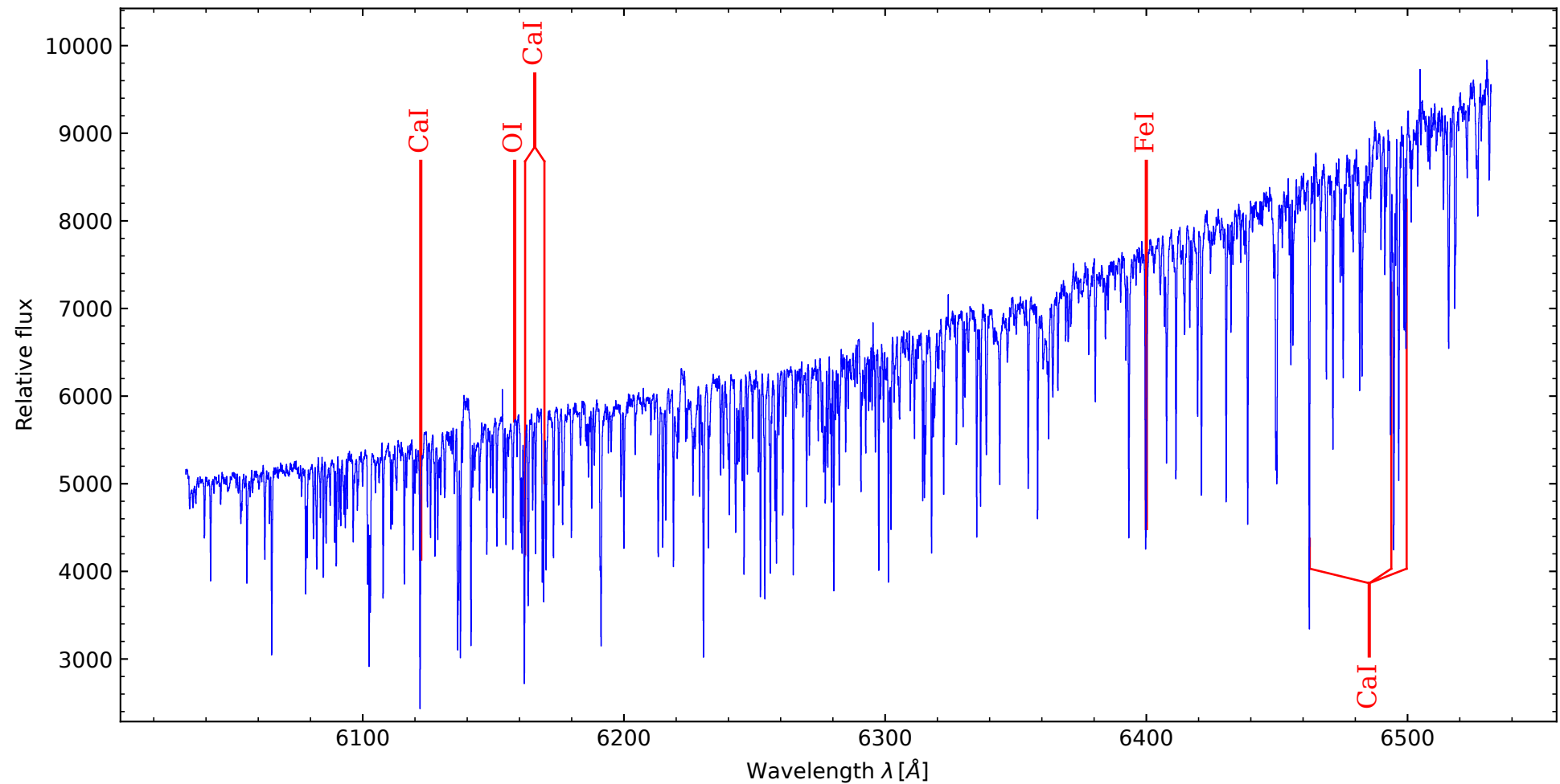
Mu Pegasi - G8 III (6032 - 6532 Å, orders merged by PYTHON)
