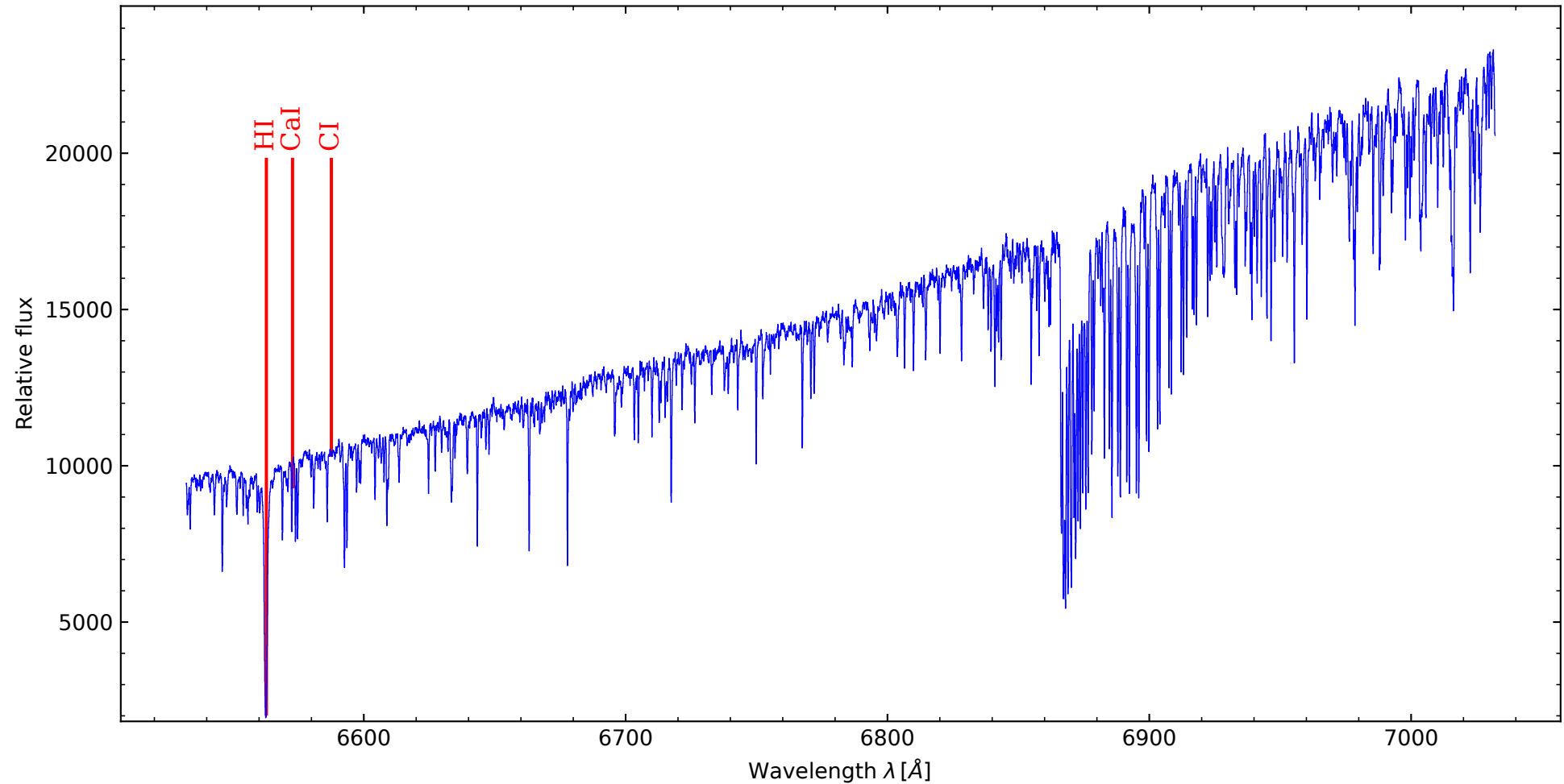
Mu Pegasi - G8 III (6532 - 7032 Å, orders merged by PYTHON)
