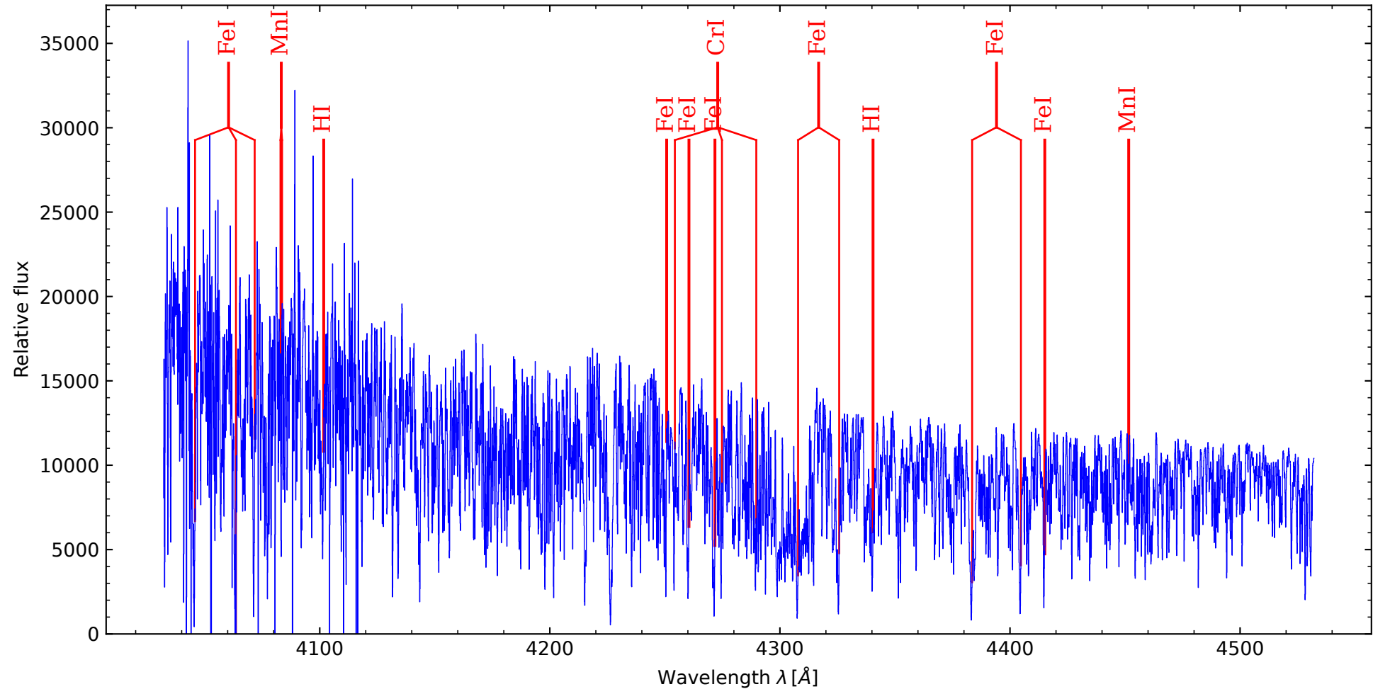
Mu Pegasi - G8 III (4032 - 4532 Å, orders merged by PYTHON)
