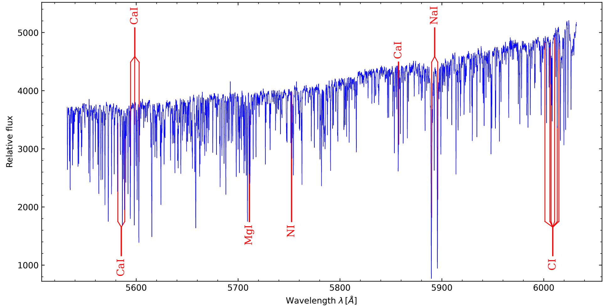
Mu Pegasi - G8 III (5532 - 6032 Å, orders merged by PYTHON)
