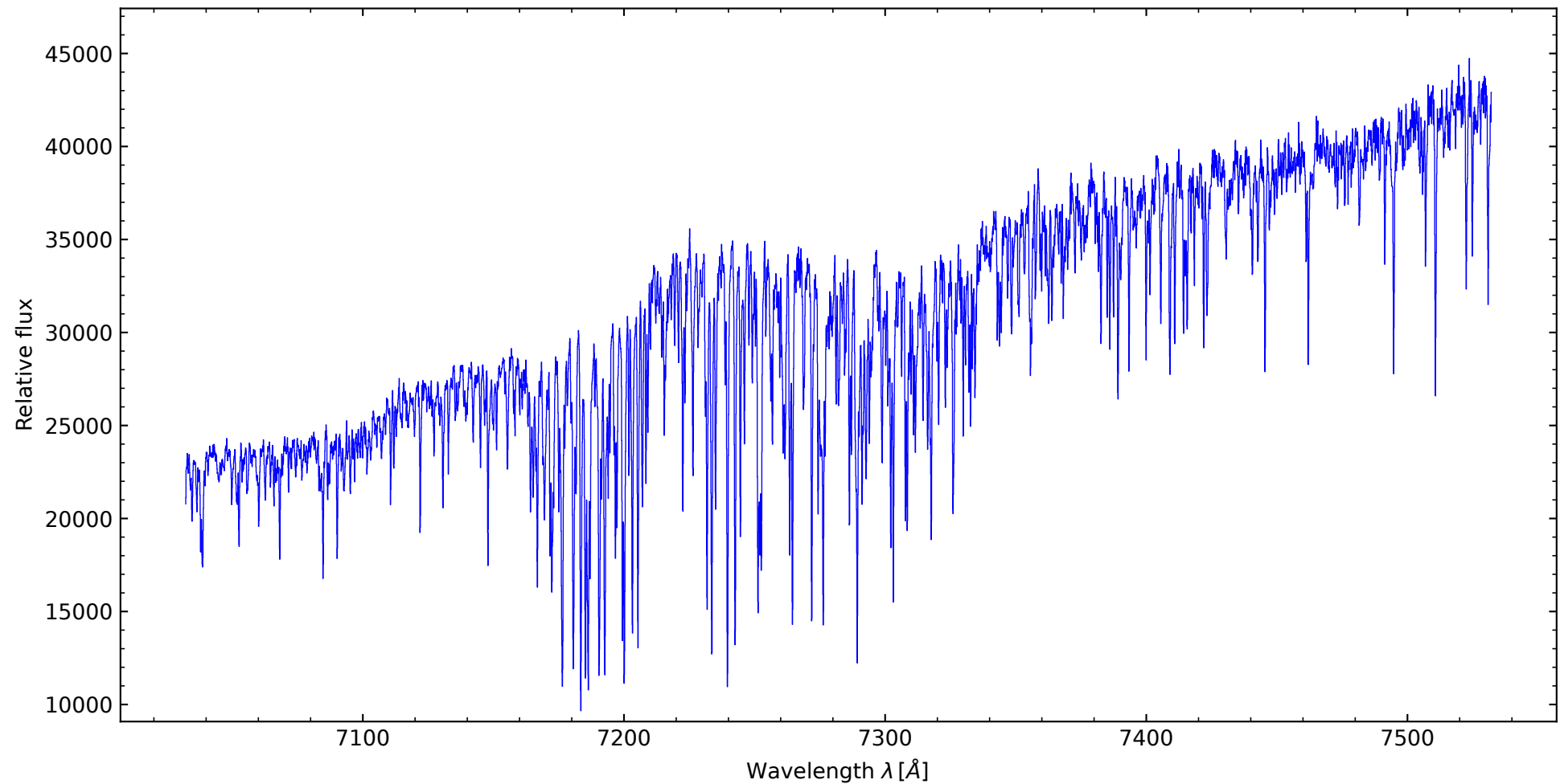
Mu Pegasi - G8 III (7032 - 7532 Å, orders merged by PYTHON)
