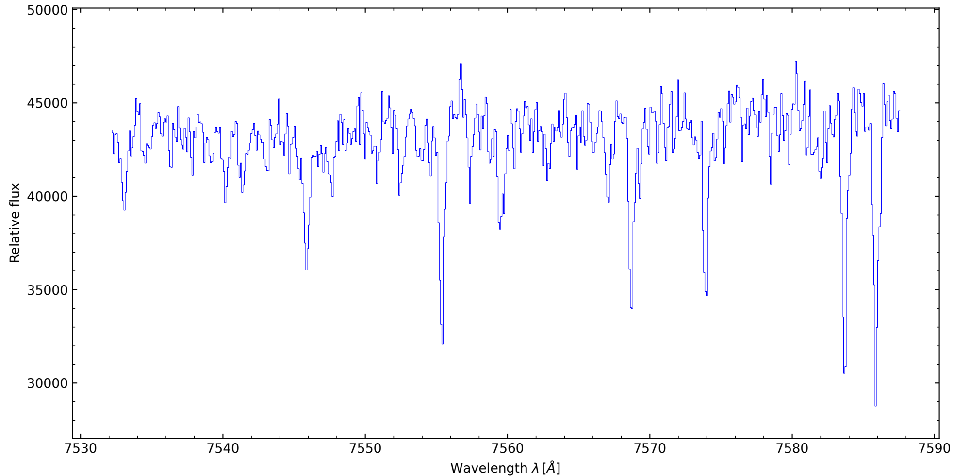
Mu Pegasi - G8 III (7532 - 7587 Å, orders merged by PYTHON)
