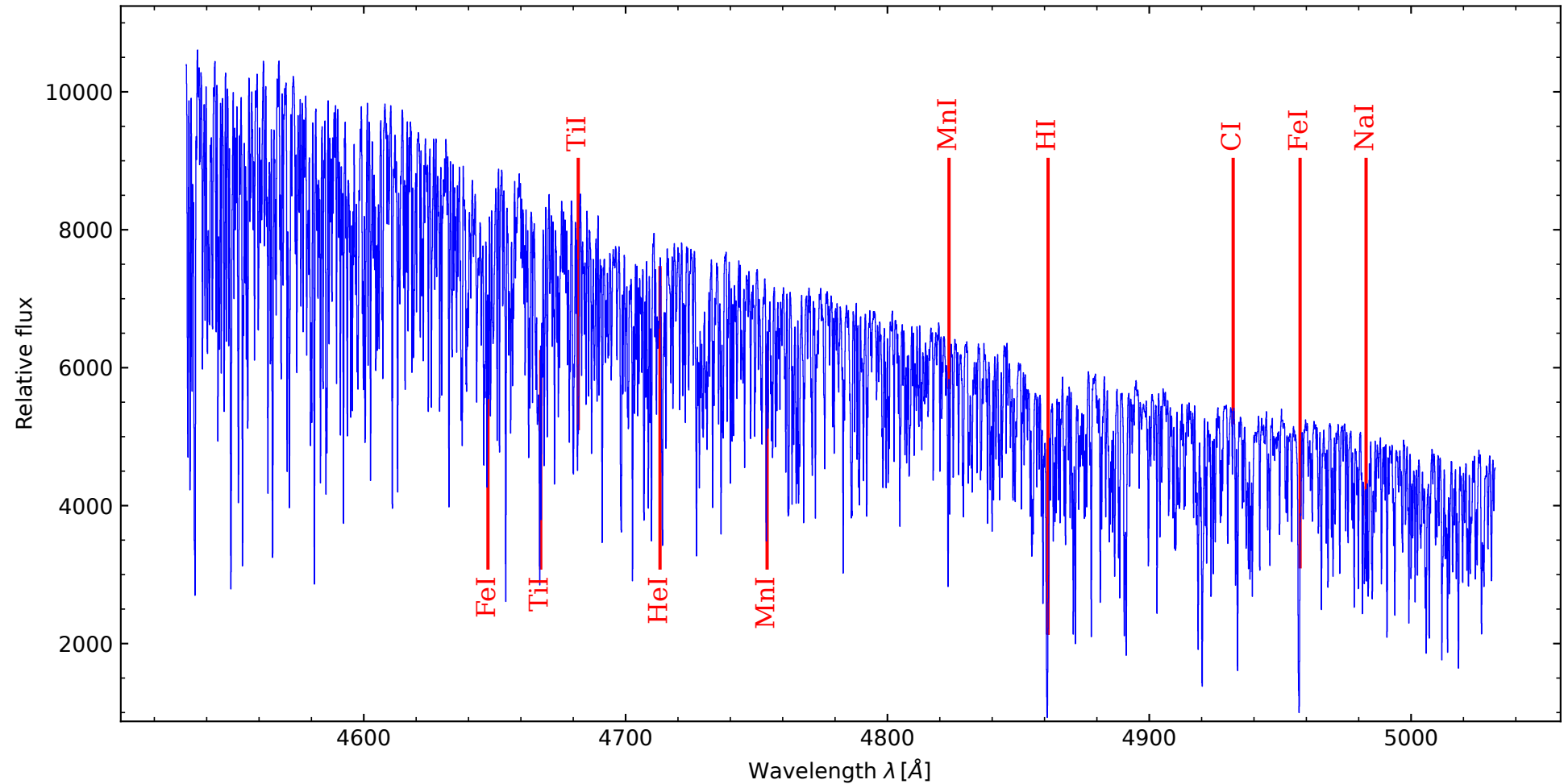
Mu Pegasi - G8 III (4532 - 5032 Å, orders merged by PYTHON)
