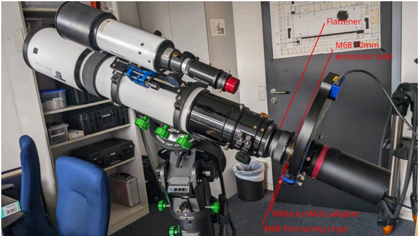
APO with flattener, QHY600 with Filter Wheel and Off-Axis Guider, and all necessary adapters
