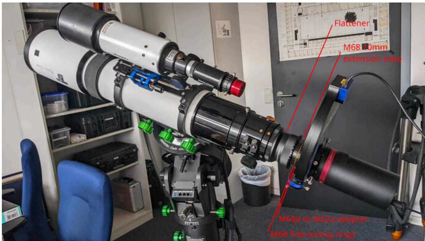
APO with flattener, QHY600 with Filter Wheel and Off-Axis Guider, and all necessary adapters
