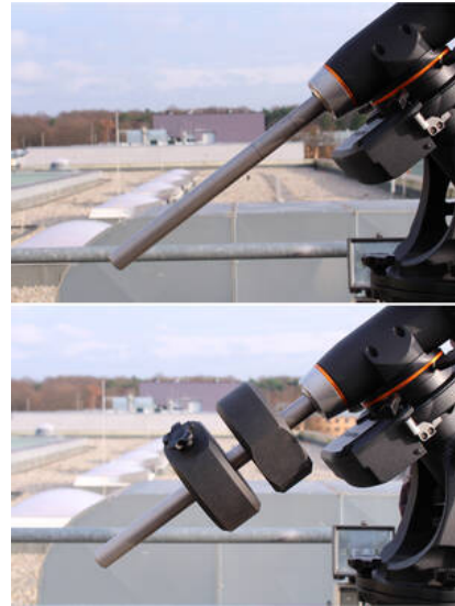
Fig. 6: CGE PRO with counterweights on bar
