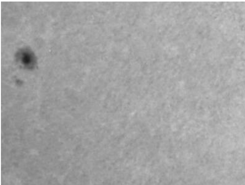
Sunspots
