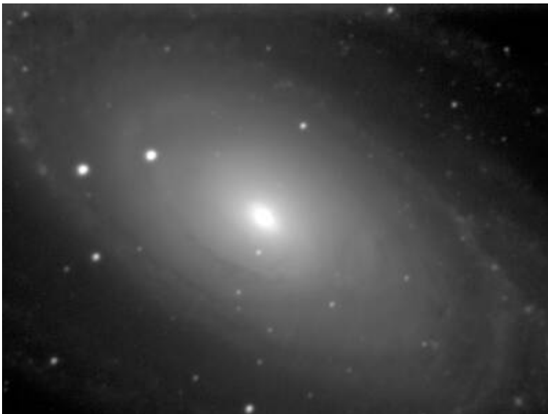
M 81
