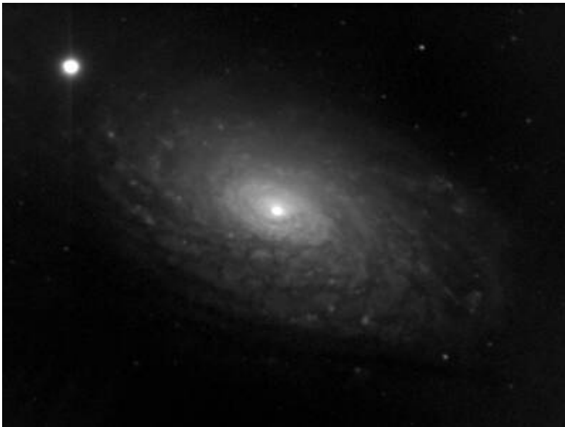
M 63
