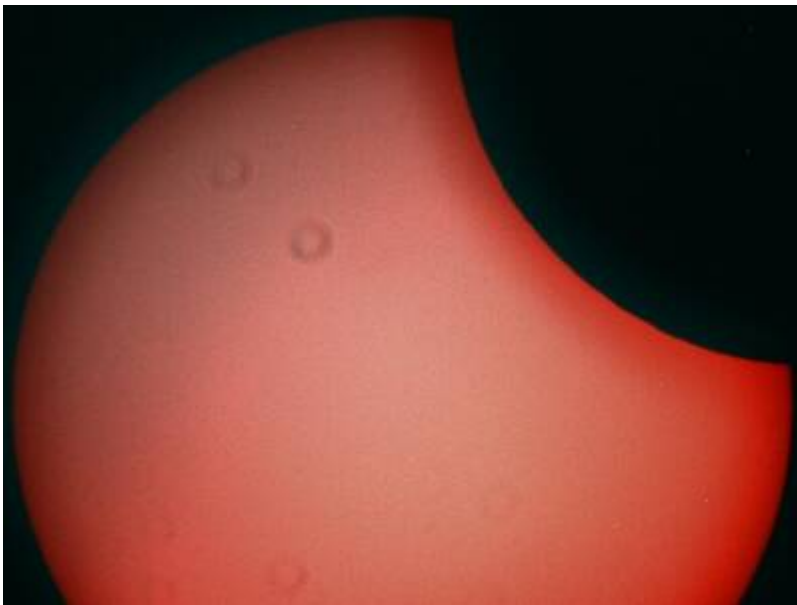
Solar eclipse
